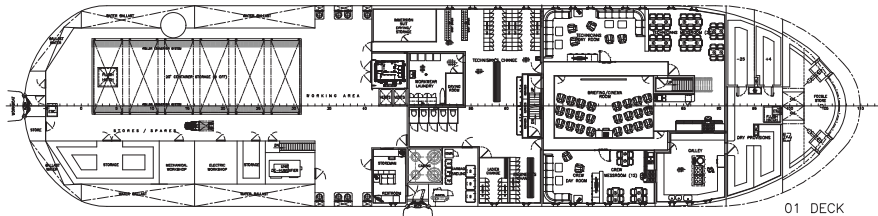
01 DECK
