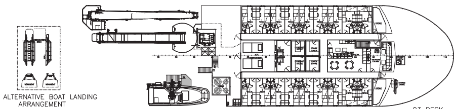
03 DECK
