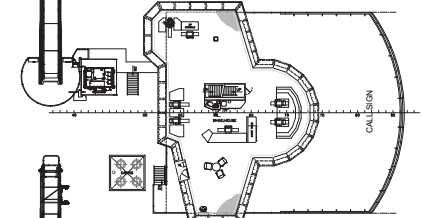
05 DECK
