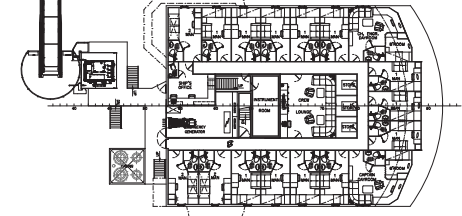
04 DECK
