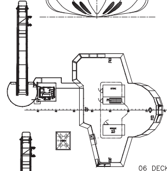
06 DECK
